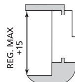
PT FLAT/ROUND (ONLY FOR ALUMINIUM)
